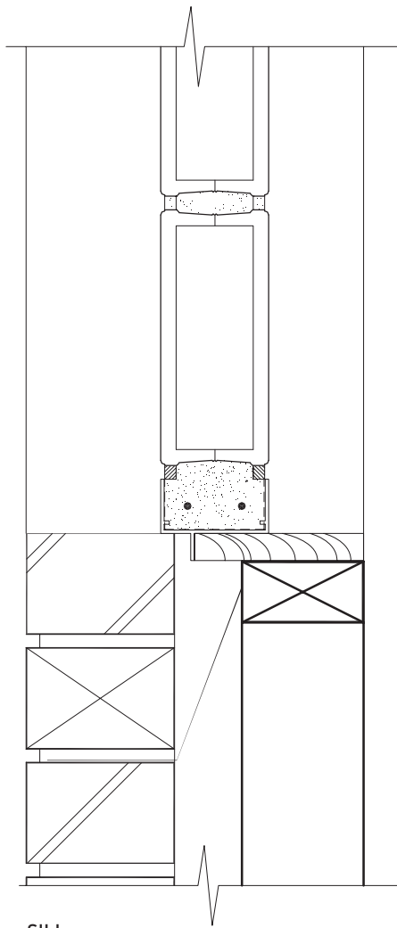
SILL
